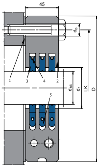
LPW-100-3 with 3 seal rings
