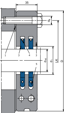
LPW-100-2 with 2 seal rings
