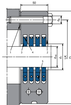
LPW-100-4 with 4 seal rings
