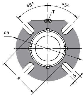
Seal cover
